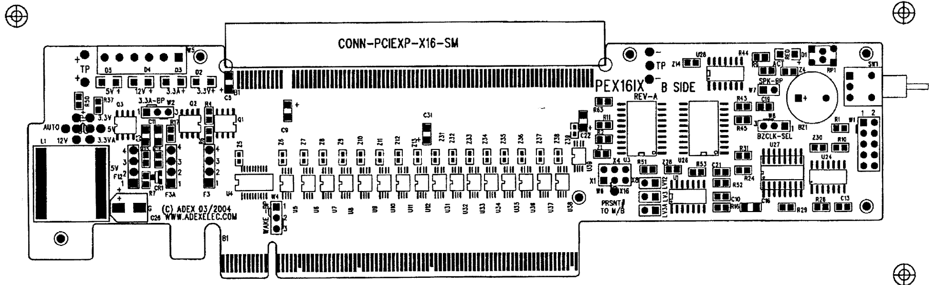
PEX16IX-A COMPONENT SIDE OUTLINE
